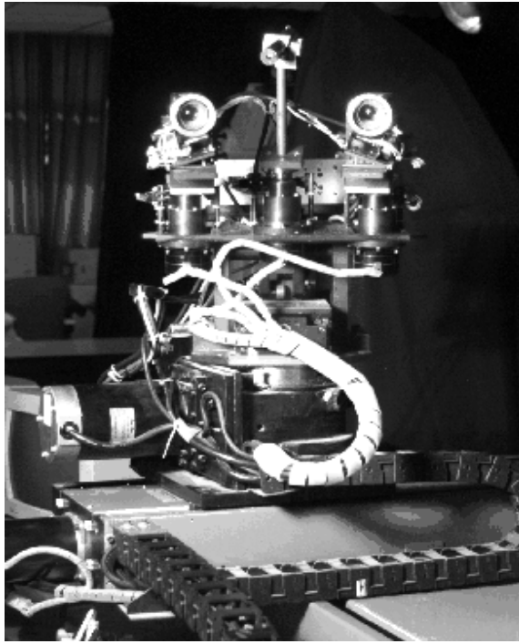
Fig. 7. A picture of the IIS head.
