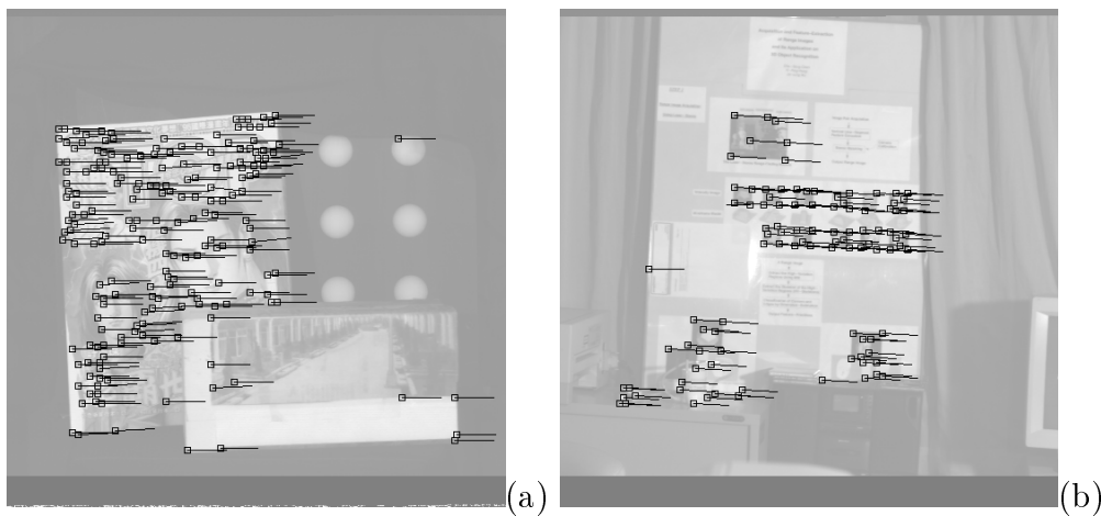
Fig. 10. (a) The optical flow field obtained from the left camera. (b) The optical flow field obtained from the right camera. The optical flow vectors in the figures are enlarged by a factor of two.
