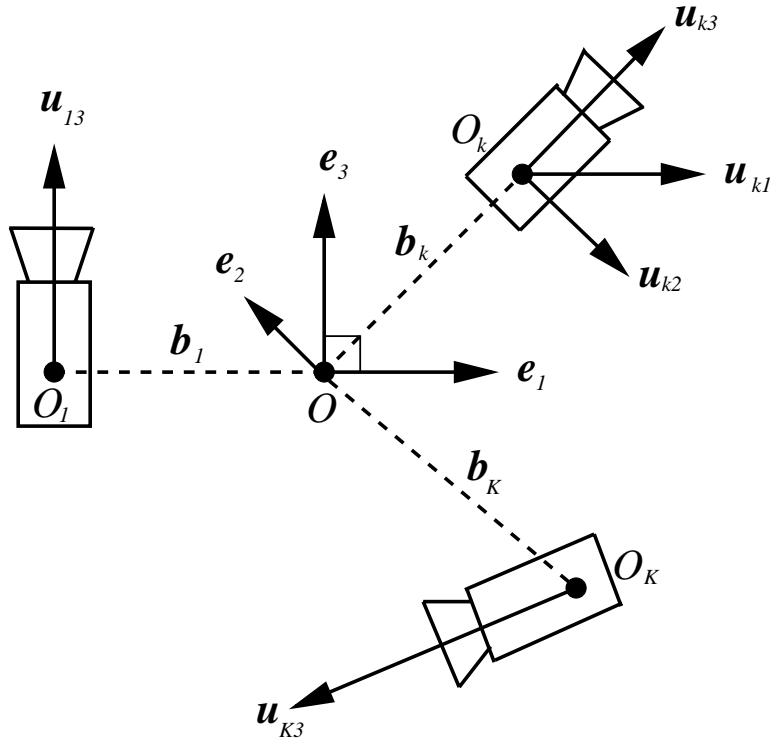
Fig. 1. An arbitrary configuration of K cameras.
