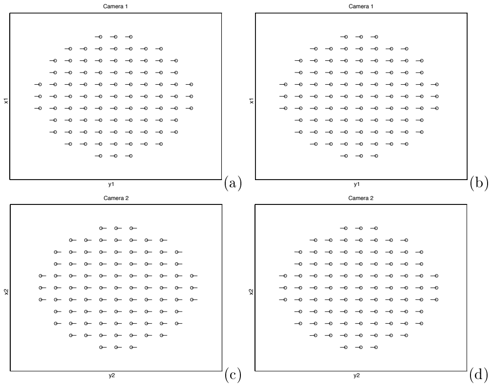
Fig. 3. (a) and (b) are the optical flow fields of the camera 1 when the vehicle is translating (a) and rotating (b). They look very similar and it is difficult to distinguish between them. (c) and (d) are the optical flow fields of the camera 2 when the vehicle is translating (c) and rotating (d). Considering the optical flow fields from both the cameras together, their scales are the same in two kind of motions but the directions are opposite only in pure translation motion.
