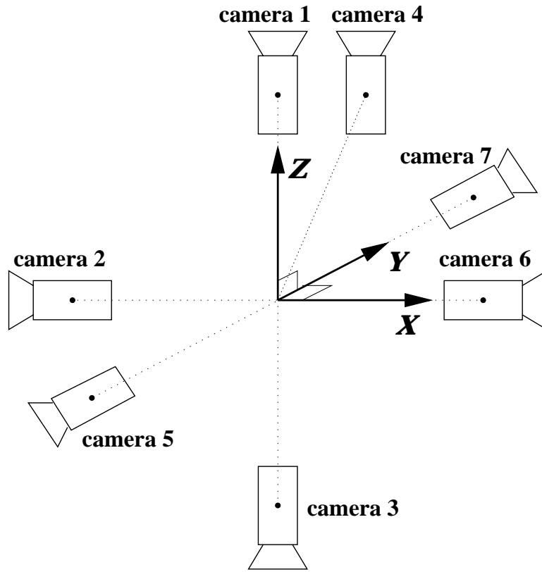
Fig. 6. The seven cameras used for the simulation of camera placement.
