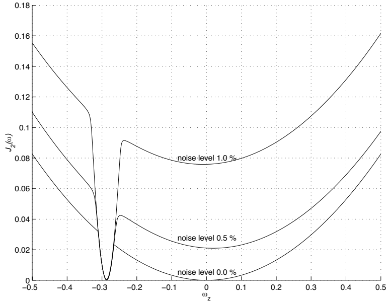
Fig. 4. The residual function J_2(\omega) by using the optical flow field of camera 1 from \omega_z = -0.5 to 0.5^\circ/s . These two local minima mean that these two kinds of motion are ambiguous.
