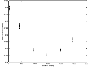
Figure 4. Residual for aperture settings.
