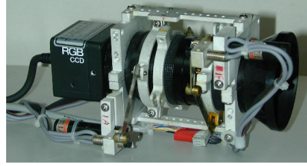
Figure 3. Our motorized zoom lens.
