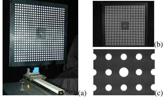
Figure 1. (a) The calibration object we used and its images acquired with (b) wide-angle and (c) telephoto zoom settings.
