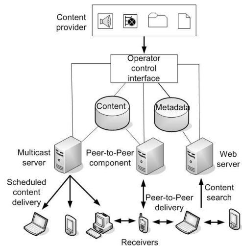
Figure 2. Architecture of the Delco system
