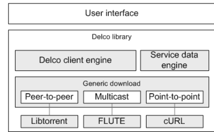
Figure 4. The architecture of the Delco client implementation
