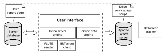
Figure 5. The architecture of the Delco server implementation
