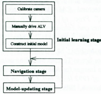
Figure 1. Illustration of the proposed “incremental-learning-by-navigation” approach
