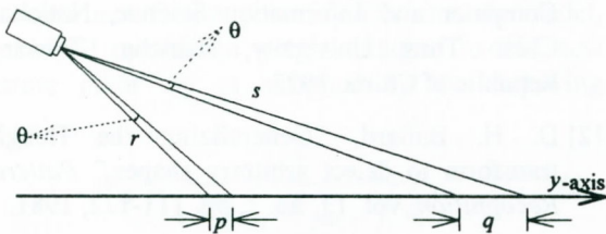
Figure 4 : Illustration of position estimation error due to the little variation of the tilt angle.
