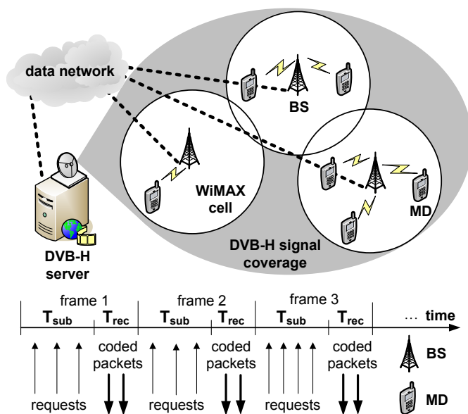
Fig. 1: Use WiMAX for packet recovery in DVB-IPDC.
