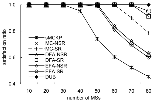
Fig. 9: The satisfaction ratio of MSs under different number of MSs, where there are 32 RSs.
