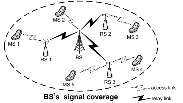
Fig. 1: The uplink communications of an 802.16j transparent-relay network.
