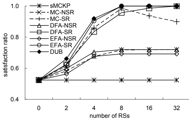
Fig. 10: The satisfaction ratio of MSs under different number of RSs, where there are 70 MSs.
