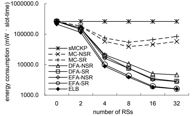
Fig. 8: The energy consumption of MSs under different number of RSs, where there are 50 MSs.
