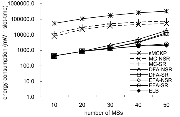
Fig. 7: The energy consumption of MSs under different number of MSs, where there are 8 RSs.
