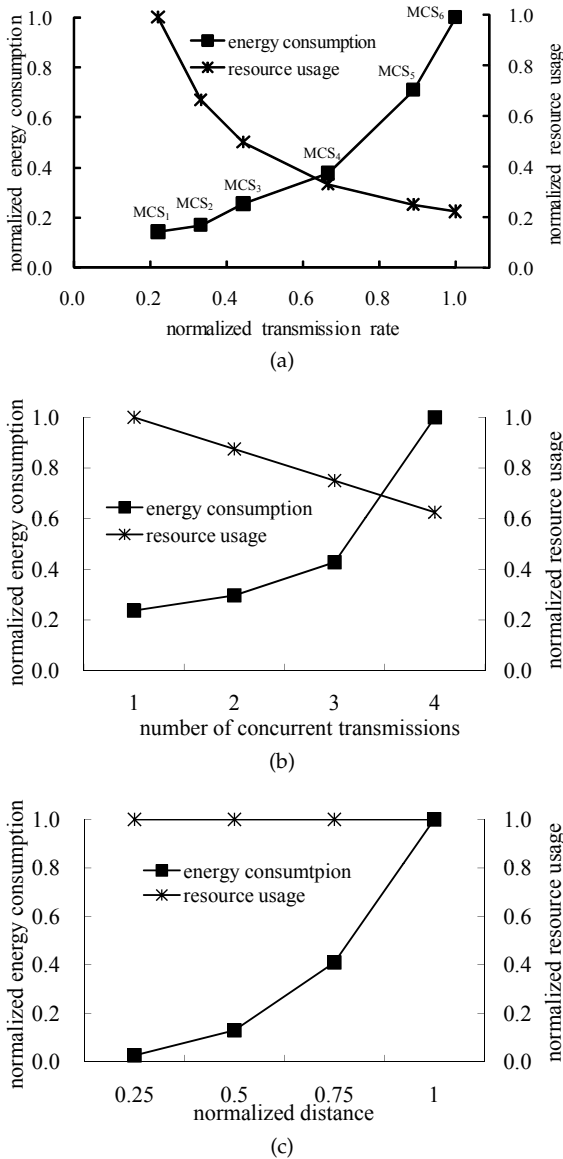
Fig. 4: The effects of rate, concurrent transmission, and receiver distance on energy consumption and resource usage.
