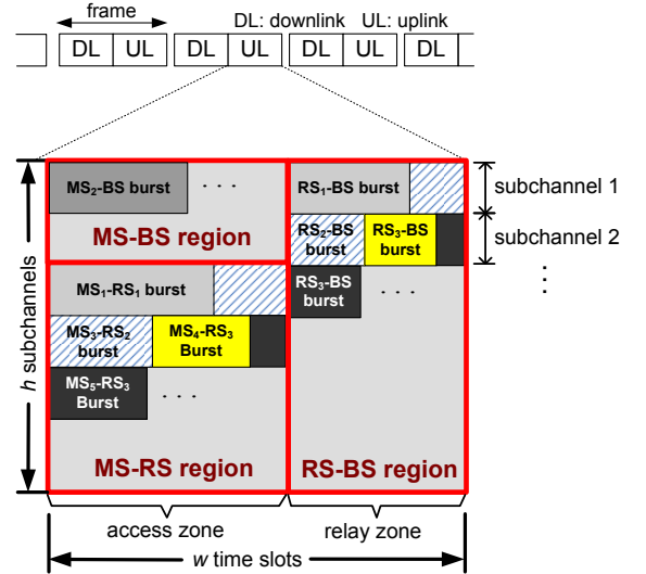
Fig. 2: The structure of the uplink subframe.
