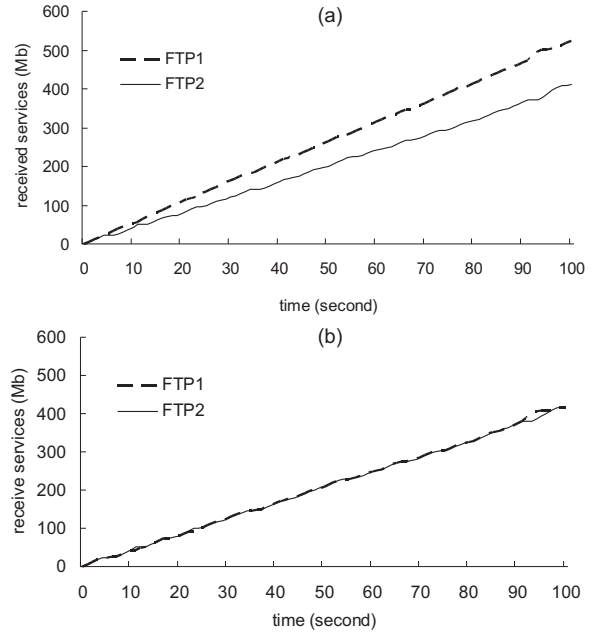
Fig. 8: Total services received by the FTP flows. (a) MR-FQ. (b) MR-FQ without considering time fairness.
