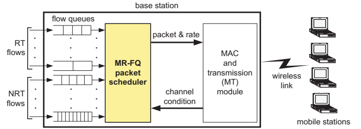
Fig. 1: System architecture of MR-FQ.
