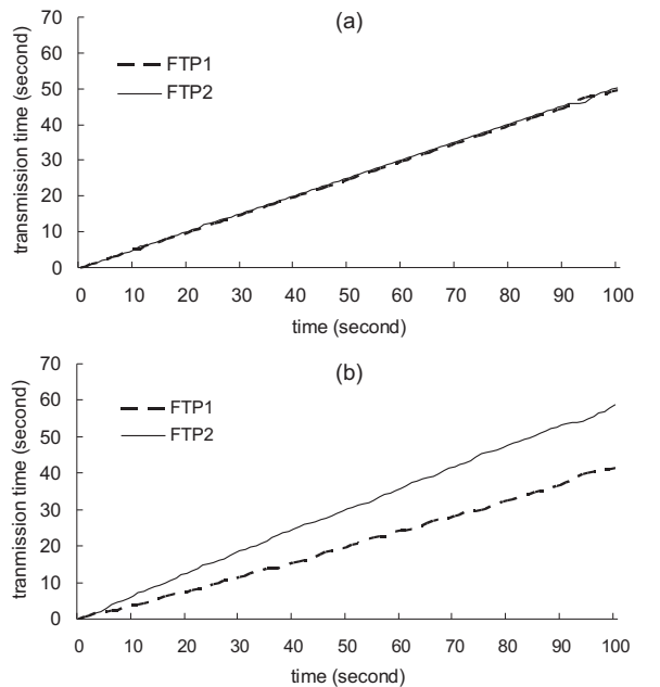
Fig. 9: Total medium time used by the the FTP flows. (a) MR-FQ. (b) MR-FQ without considering time fairness.
