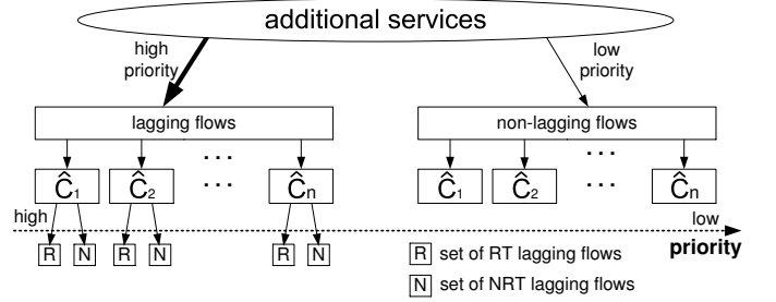
Fig. 4: Dispatching additional services in the Compensation Scheme.
