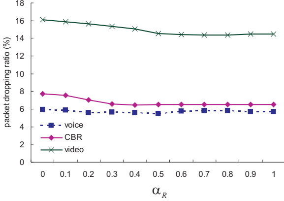
Fig. 12: Packet dropping ratios of RT flows under different \alpha_R values.
