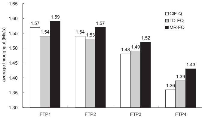
Fig. 7: Average throughput of NRT flows.
