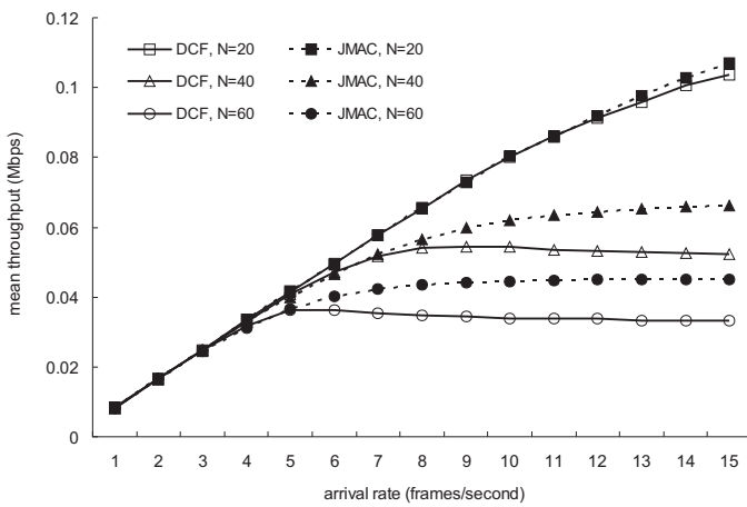
Fig. 9: Mean throughput versus frame arrival rate.
