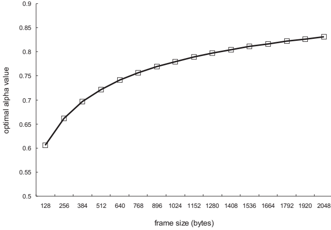
Fig. 6: Data frame size vs. the optimum alpha \hat{\alpha} .
