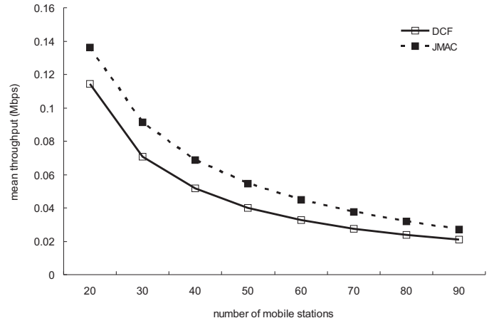
Fig. 11: Saturation mean throughput versus network density.
