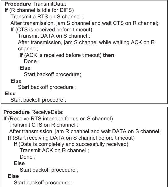
Fig. 2: The procedures of transmission and receipt of control/data frames in JMAC .
