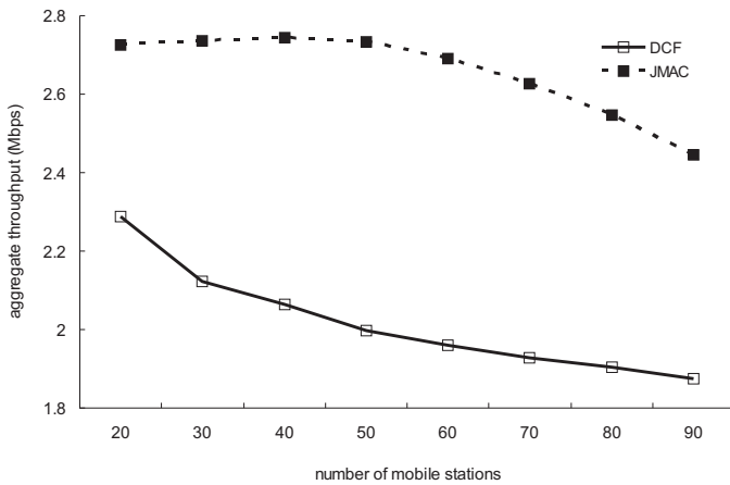
Fig. 10: Saturation aggregate throughput versus network density.
