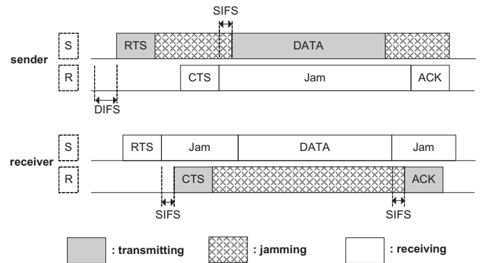
Fig. 3: The timing diagram of transmission of control/data frames.
