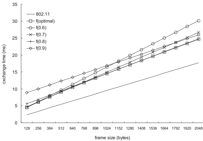
Fig. 7: Frame exchange time in IEEE 802.11 and in JMAC for different data frame sizes and different \alpha .
