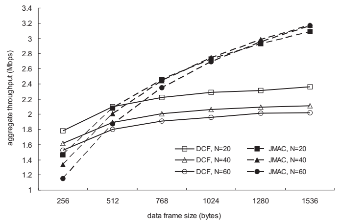
Fig. 12: Aggregate throughput versus frame size.
