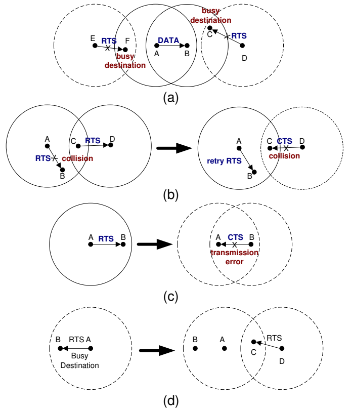
Fig. 1: Erroneous reservations caused by (a) busy destination, (b) frame collision, (c) transmission error, and (d) the problem itself.
