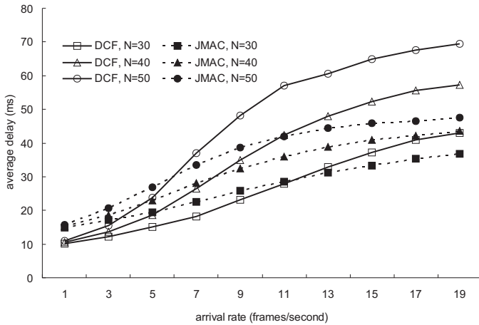
Fig. 14: Mean access delay versus frame arrival rate.
