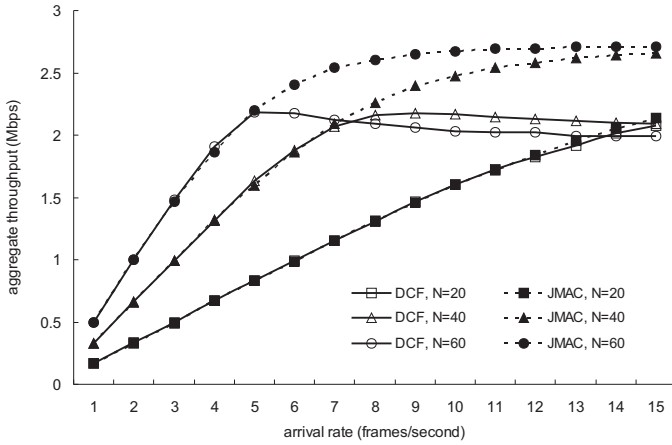
Fig. 8: Aggregate throughput versus frame arrival rate.
