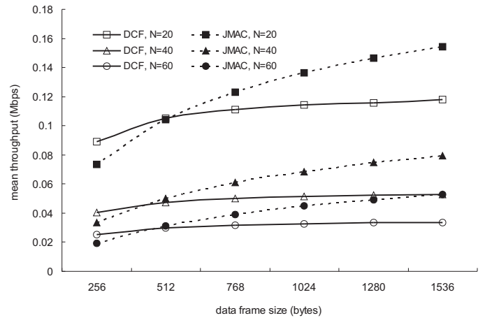
Fig. 13: Mean throughput versus frame size.
