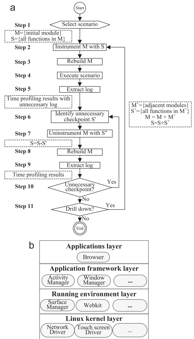
Fig. 2. Staged iterative instrumentation approach. (a) Procedure of staged iterative instrumentation profiling. (b) Major layers and modules related to Android browsing.
