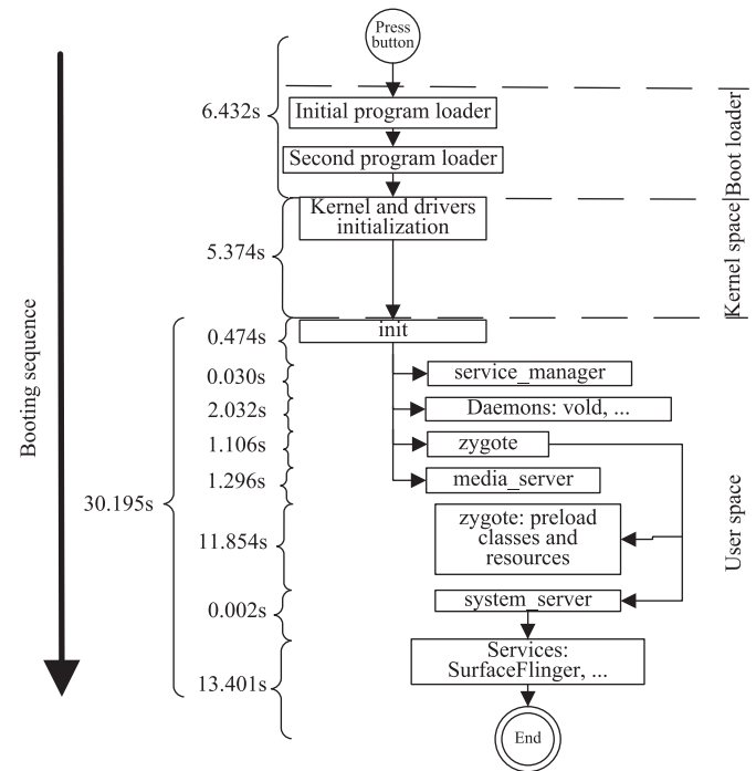
Fig. 7. Profiling results of booting procedures.
