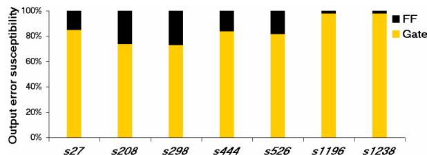
Figure 1. SER impact of internal gates and flip-flops
