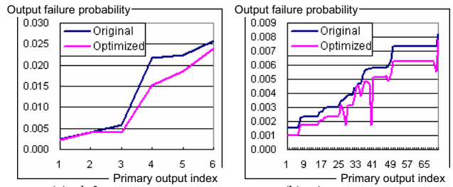
Figure 8. Output failure probabilities over all primary outputs before and after optimization by our SER reduction framework
