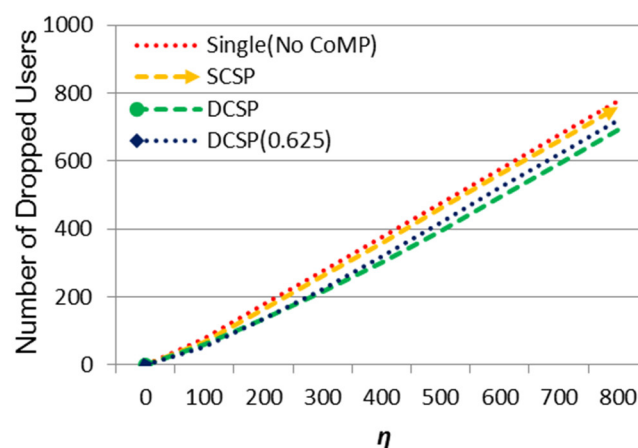
Figure 7. The effect of \eta on the number of dropped users.
