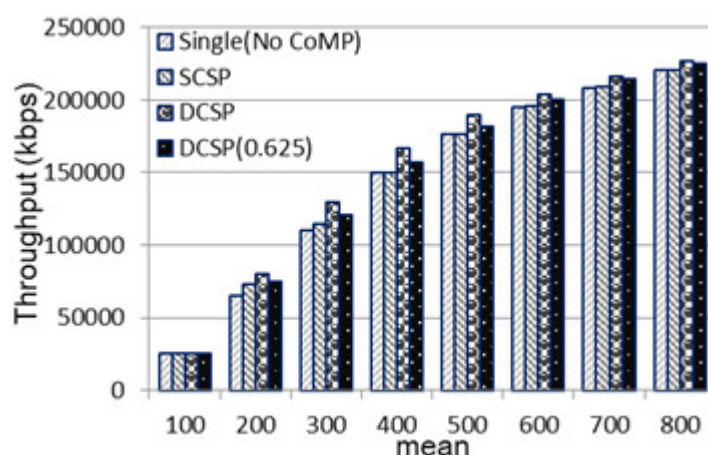
Figure 16. The effect of mean on throughput.
