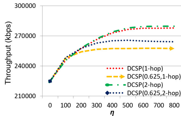
Figure 10. The effect of \eta on throughput (1-hop neighbors as candidates VS. 1-hop and 2-hop neighbors as candidates).
