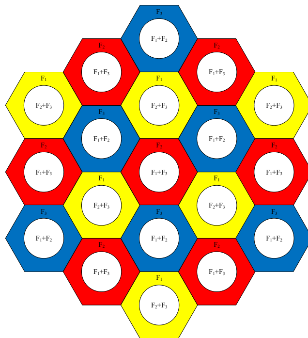
Figure 2. Deployment of base stations and channel assignment.
