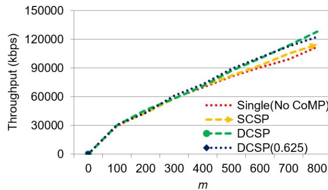
Figure 12. The effect of m on throughput.
