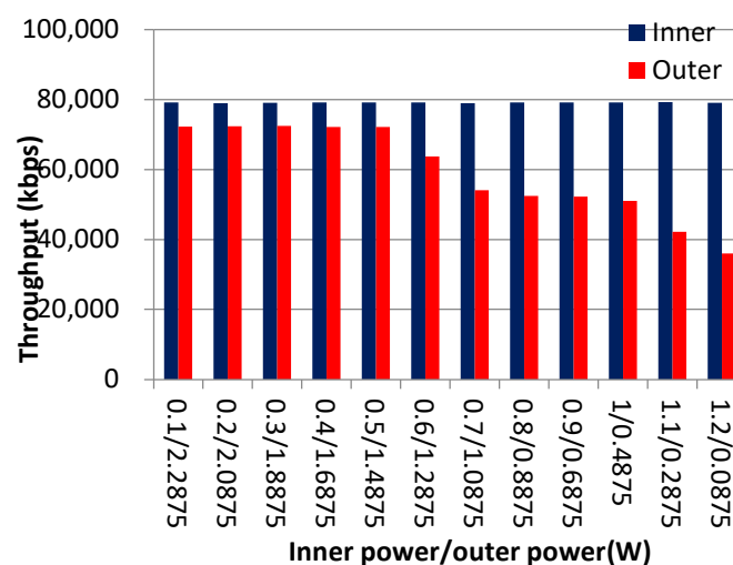
Figure 4. Power allocation VS. inner/outer area throughput.
