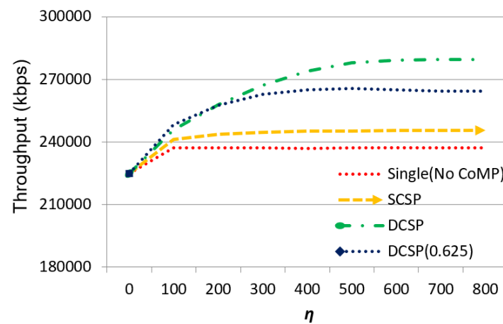
Figure 6. The effect of \eta on throughput.
