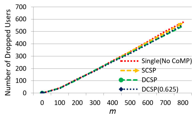
Figure 13. The effect of m on the number of dropped users.
