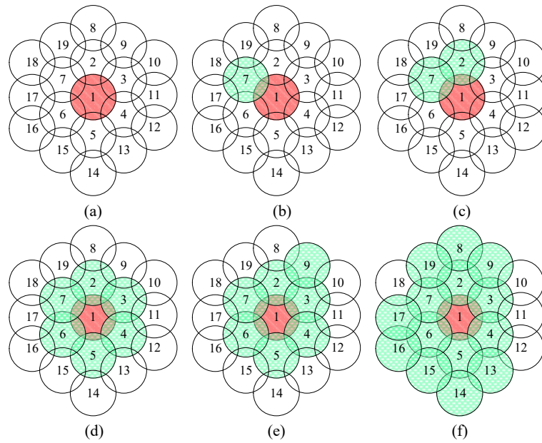
Figure 3. An example of dynamic cooperating set planning.
