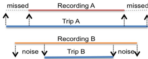
Fig. 4. (Top) Completeness of recordings measures the percentage of a trip being recorded and labeled. (Bottom) Precision of recordings measures the percentage of a recording that precisely reflects its label.
