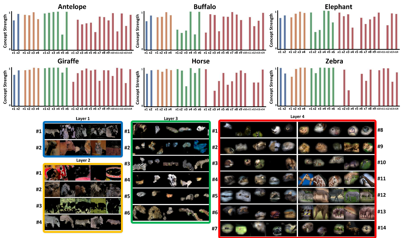
Figure 16. Class-wise explanation. For each category, the explanation is derived by aggregating the MCP distributions for the images of the target class. The concept strength indicates whether the concept prototypes are prevalent in most images belonging to the same class in the dataset.
