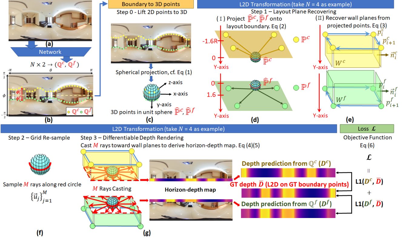
Figure 4. The overall framework of our proposed LED 2 -Net. Our layout estimation network takes (a) a RGB panorama as input, and outputs (b) the layout representation which is composed of two sets of layout boundary points ( \mathbb{Q}^c, \mathbb{Q}^f ) on the ceiling and the floor respectively. Our novel L2D (layout-to-depth) transformation is applied to transform the layout representation, which are first (c) lifted to 3D space (cf. Section 3.1), into the horizon-depth maps (i.e. D^c and D^f ). The L2D transformation is composed of three main steps: (d)(e)“Layout Plane Recovering” (cf. Section 3.2) to recover the plane equation (i.e. W^c and W^f ), (f) “Grid Re-sample” (cf. Section 3.2), and (g)“Differentiable Depth Rendering” (cf. Section 3.2). The training objective of our LED 2 -Net is thus defined by the errors between our estimated horizon-depth maps and the corresponding ground truth \bar{D} (cf. Section 3.3).
