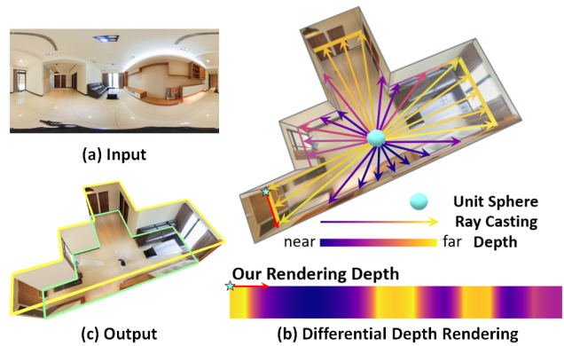
Figure 1. Our LED 2 -Net takes the (a) single panorama as input and infers the (c) 3D room layout. We propose the (b) Differential Depth Rendering technique to incorporate the geometry-aware information into our model.
