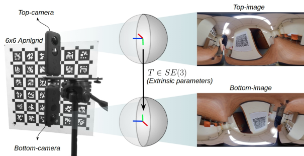
Fig. 3: Our 360° stereo system composed of two Insta360® ONE X cameras. In order to align both equirectangular images (top and bottom), the extrinsic parameters between the cameras is needed. This transformation is obtained by stereo calibration.
