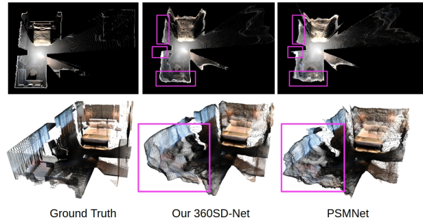
Fig. 5: Qualitative point cloud comparison between 360SD-Net (Ours) and the PSMNet. Our model shows a better geometry estimation with less distortion and a more accurate structure.
