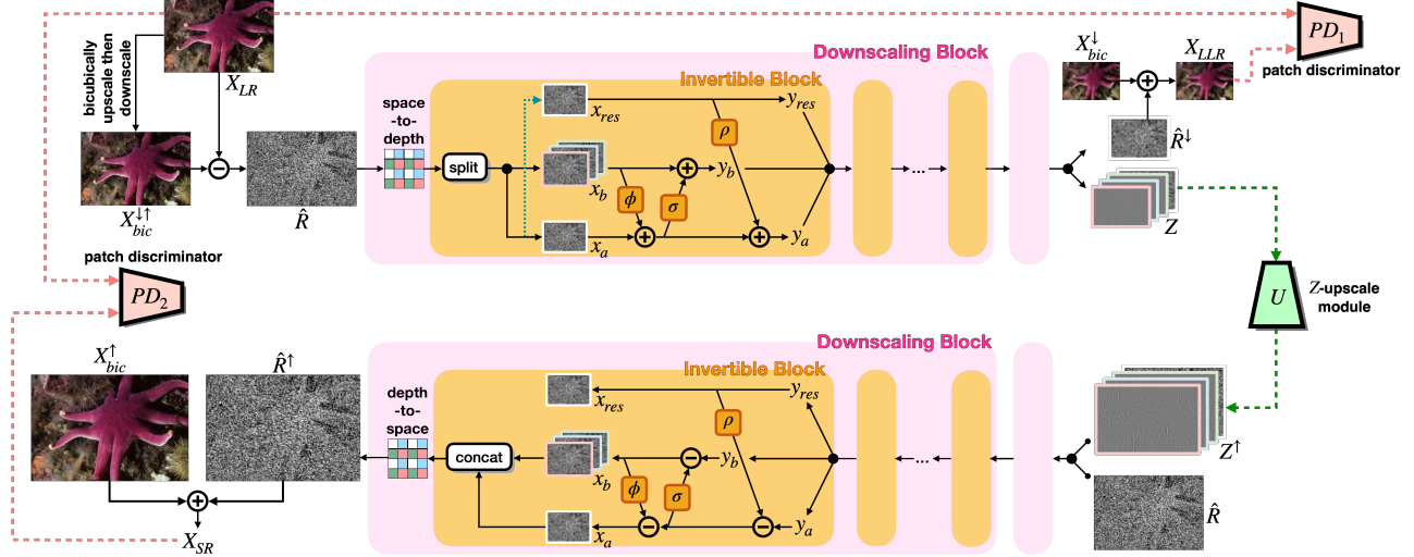
Fig. 1: Illustration of our proposed framework for zero-shot blind image super-resolution.
